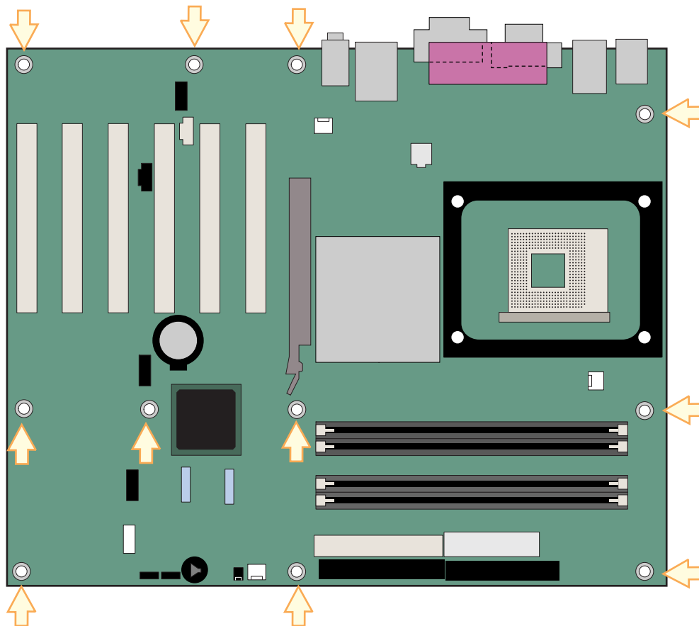
Figure 4. Location of Desktop Board Mounting Screw Holes
